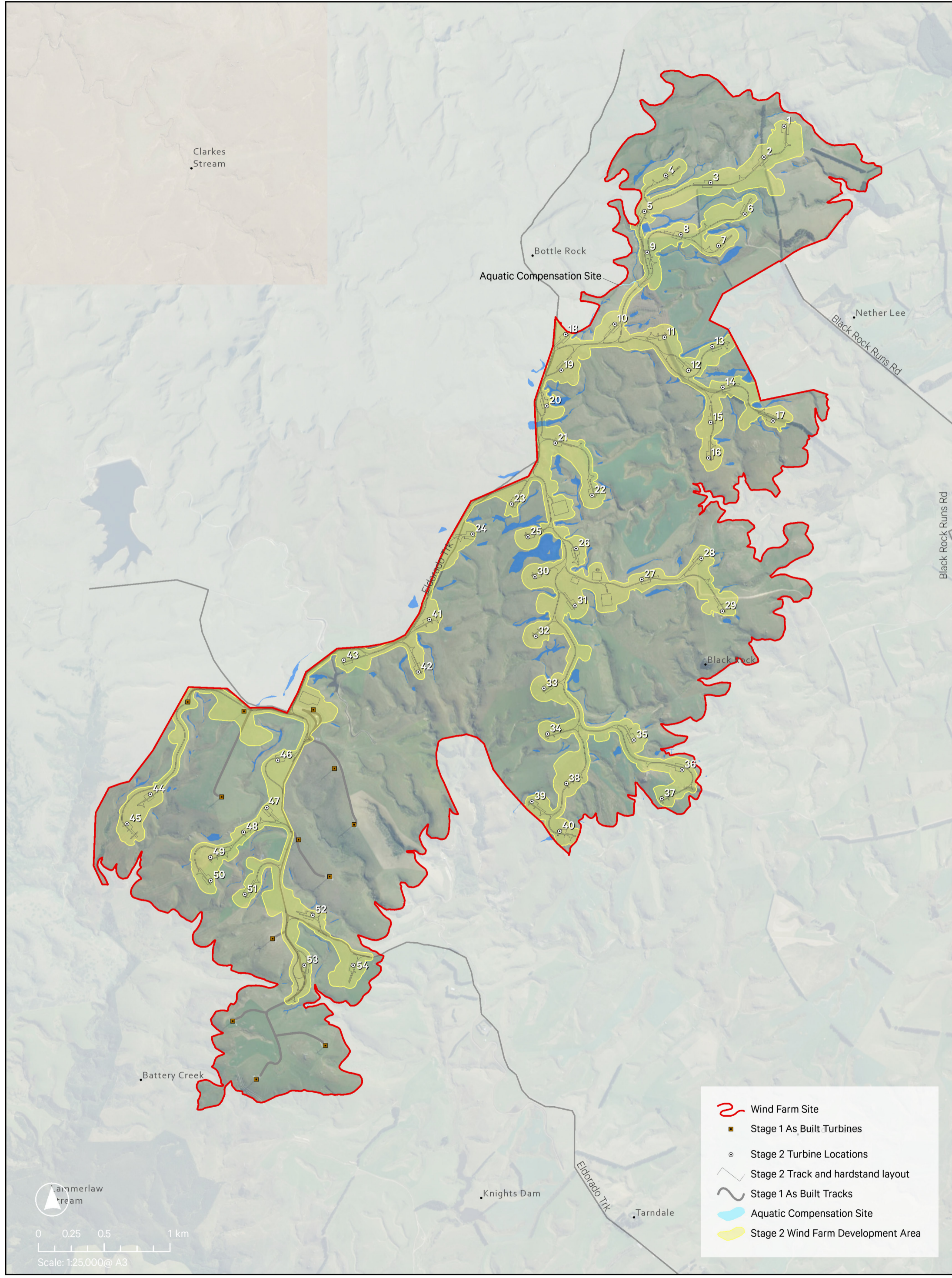
Map 1 - Puke Kapo Hau Stage 2 Layout Plan
